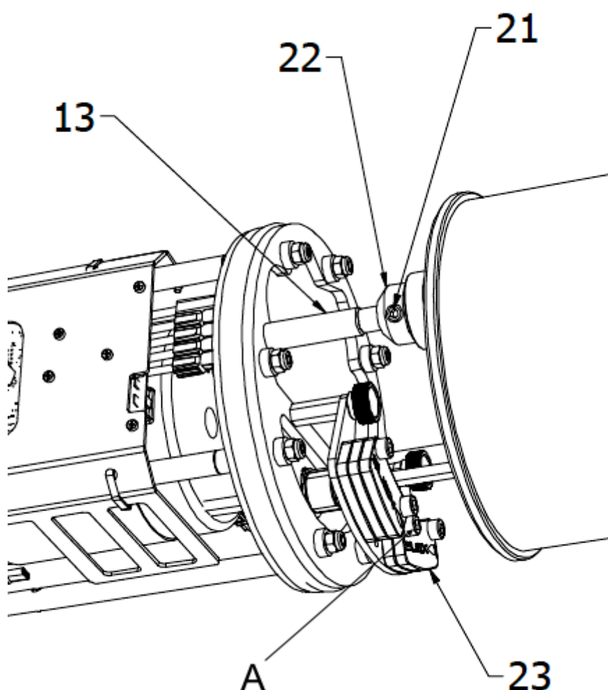
Fig. 8a (view of the scooter without the outer casing)
