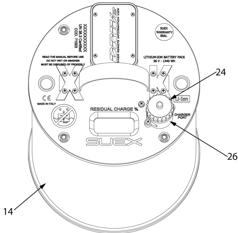
Fig.4 - Battery charging
