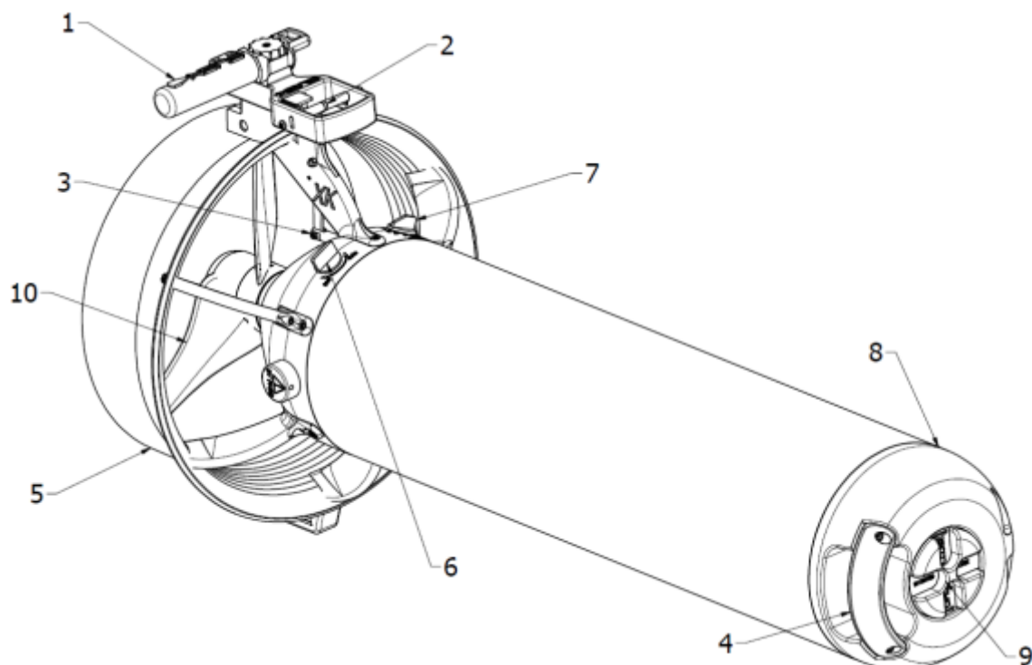
Fig. 1 - Part description
