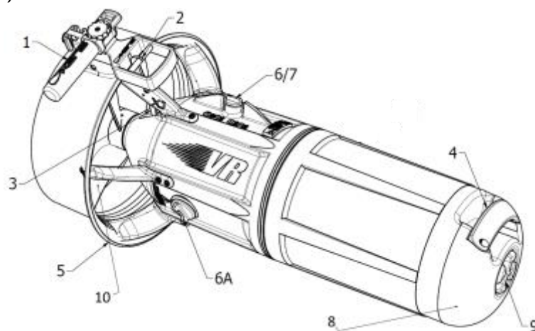
Fig. 1 - Part description
