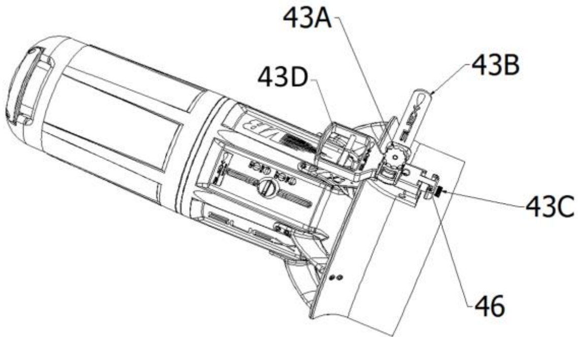
Fig.4 - Revolving handle
