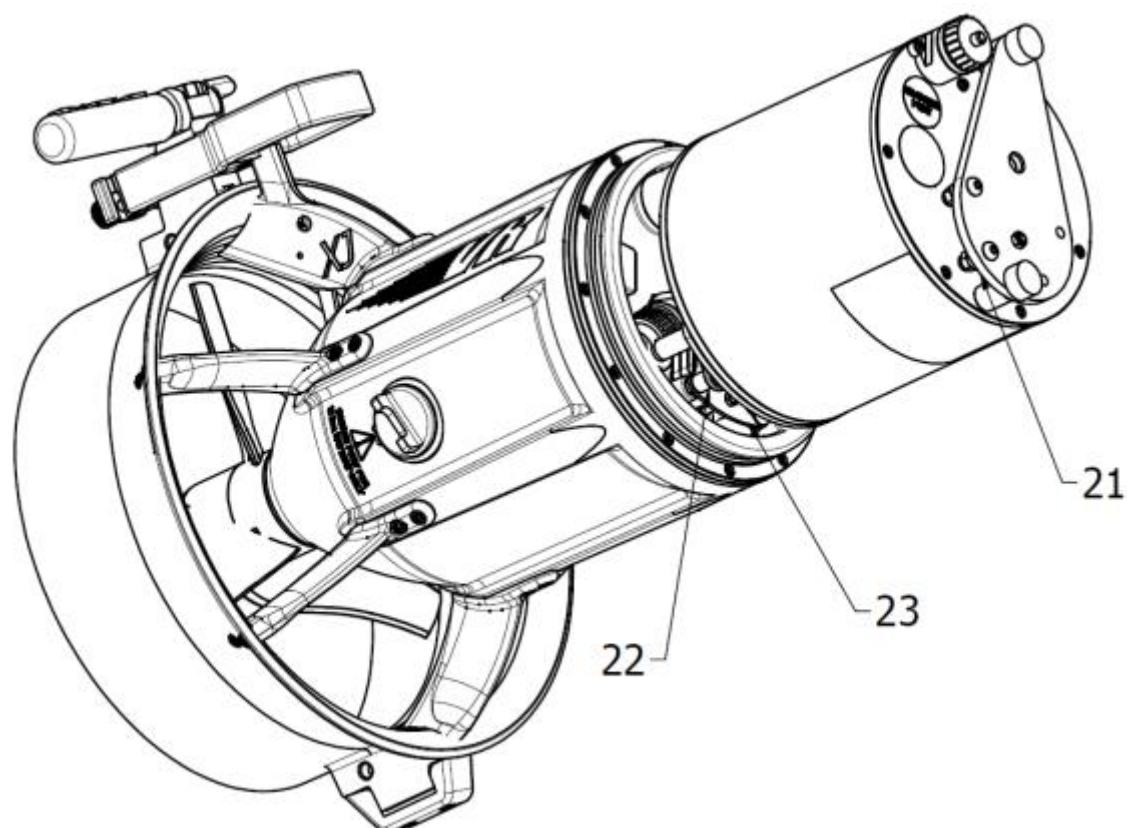
Fig.7 - Ballast insert
