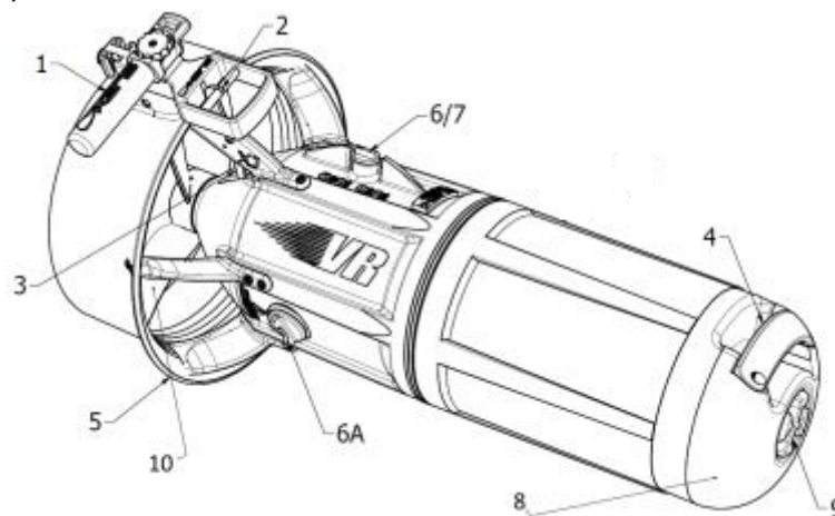
Fig. 1 - Part description
