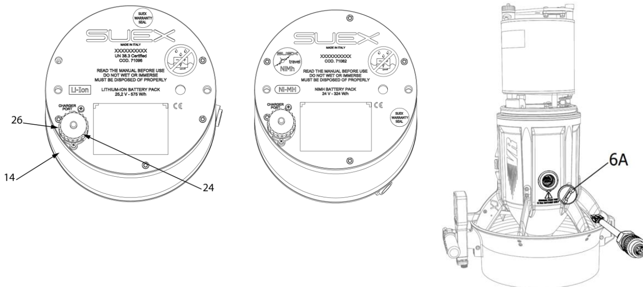
Fig.4 - Battery charging
