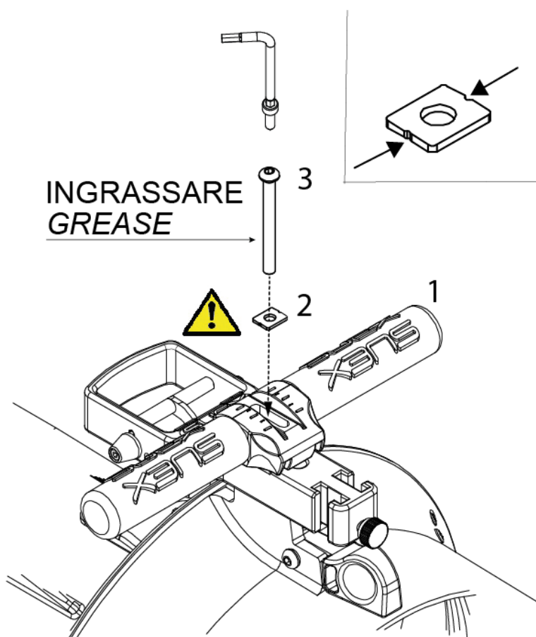
Fig 6 - Handle installation
