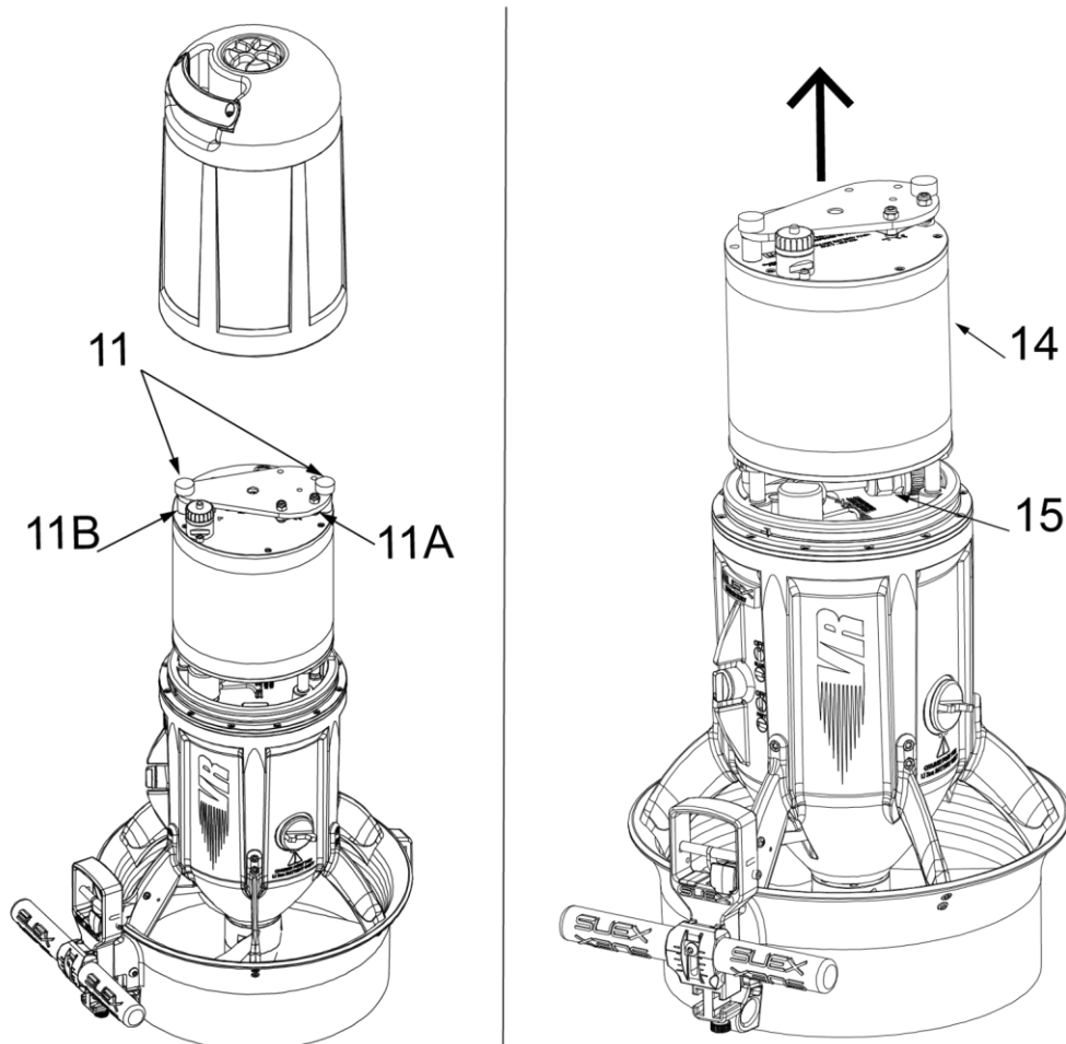
Fig 24 - Battery compartment opening
