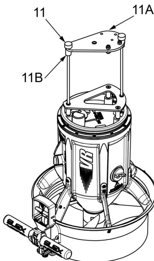
Fig 27 - Plate removal
