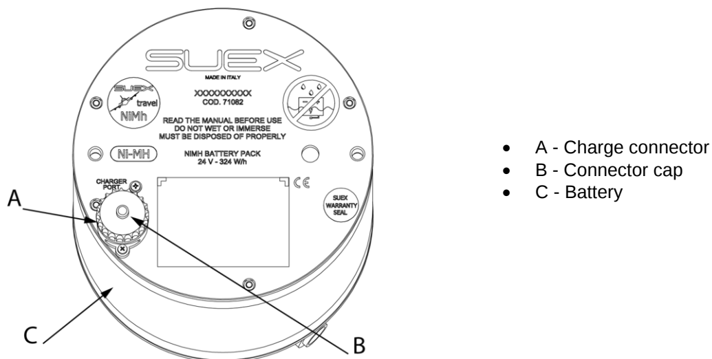
Fig 25 - VRT - NiMh battery
