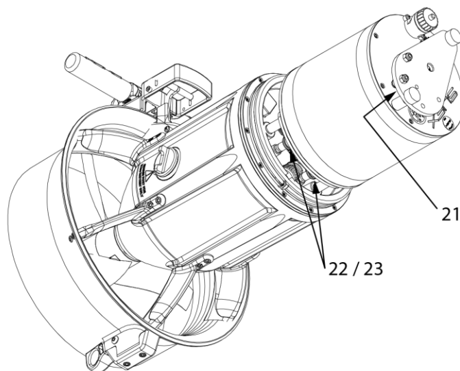
Fig 14 - Ballast insert
