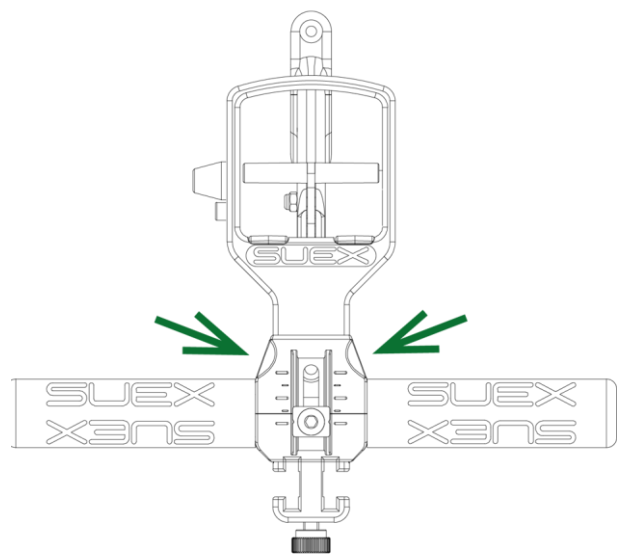
Fig 8 - Installation opposite handle
