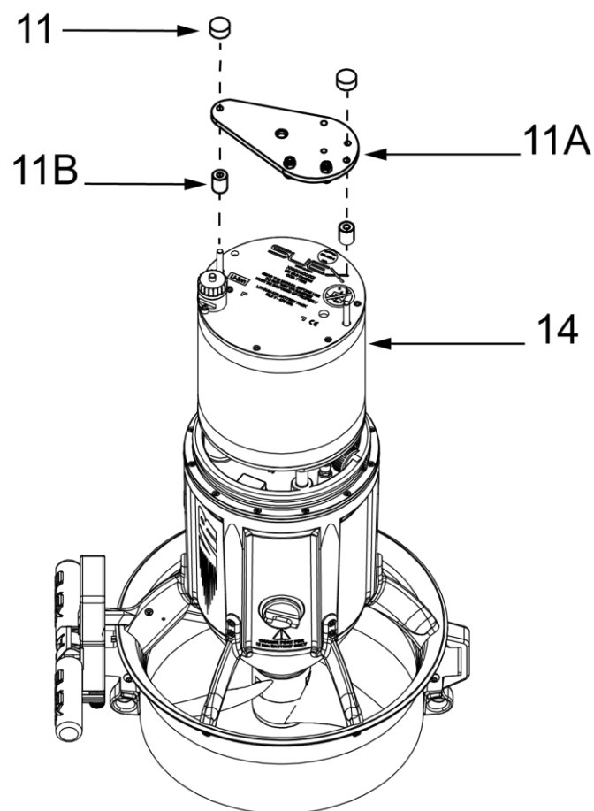
Fig 29 - Battery inserting
