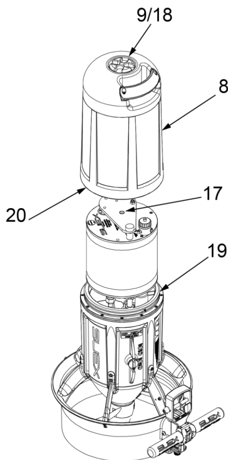
Fig 30 - Closing the battery compartment
